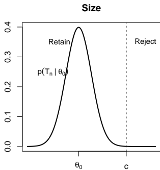
T under the null hypothesis
