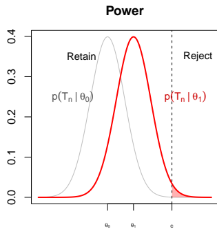
T under an alternative
